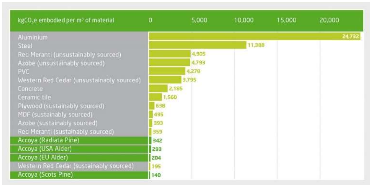
Figure 22: Embodied energy of common building materials
